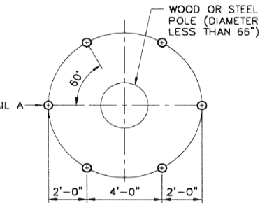
PLAN TYPICAL WOOD OR STEEL POLE PROTECTION C9520.12
