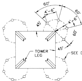
PLAN TYPICAL TOWER LEG PROTECTION C9520.11
